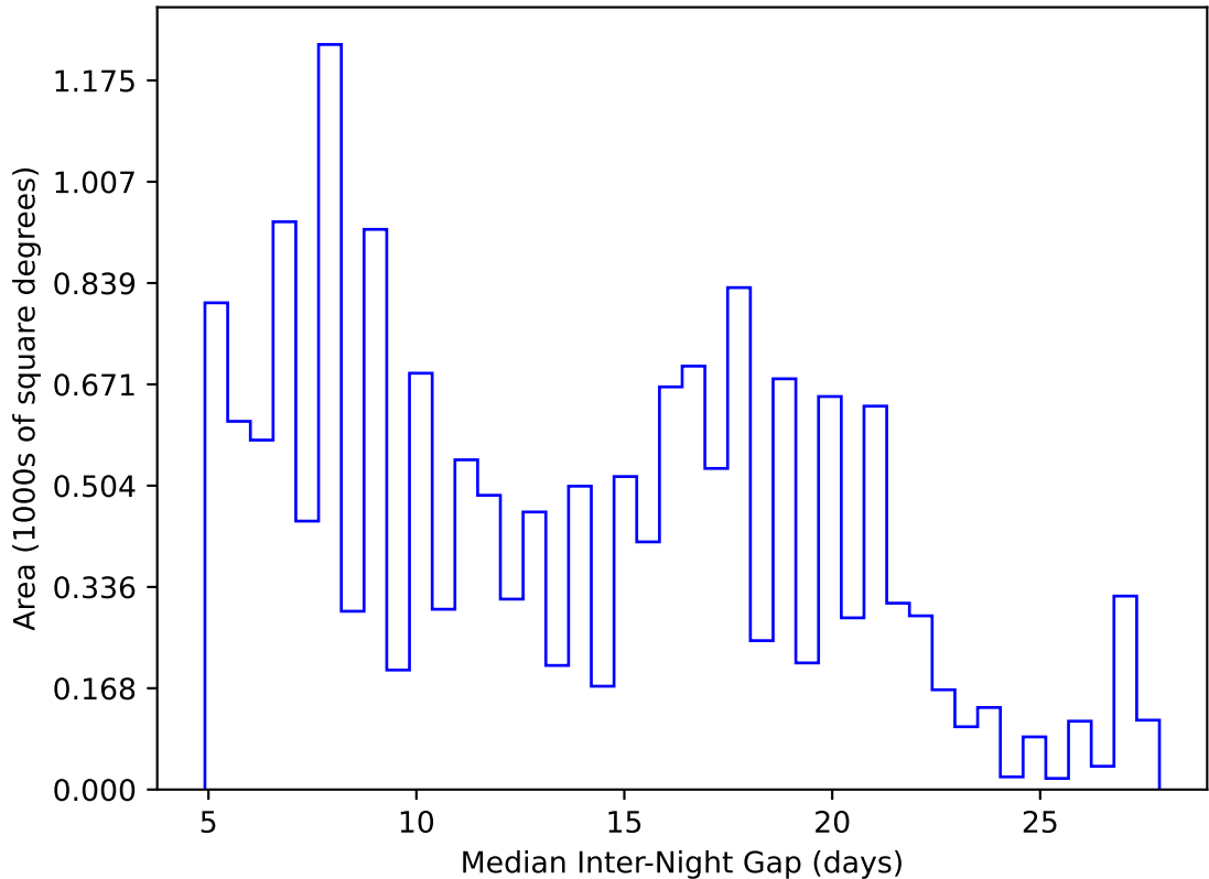
too_elab_2yr_r64_d3_ugrizy_v3.4_10yrs WFD y band: Median Inter-Night Gap
