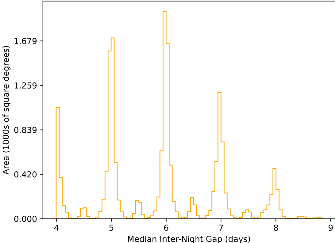
too_elab_2yr_r64_d3_ugrizy_v3.4_10yrs WFD r band: Median Inter-Night Gap
