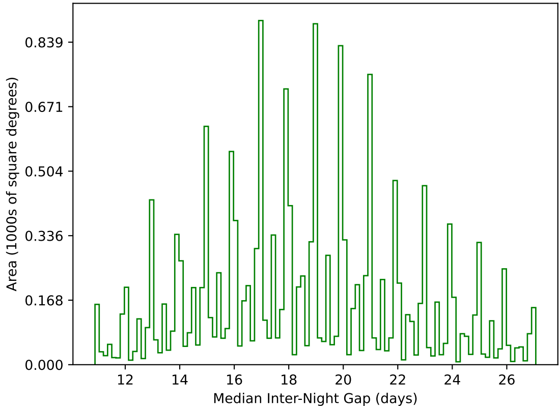
too_elab_2yr_r64_d3_ugrizy_v3.4_10yrs WFD g band: Median Inter-Night Gap
