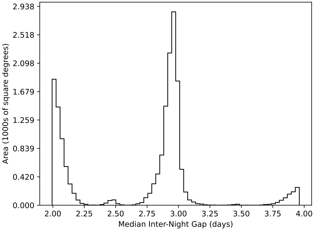
too_elab_2yr_r64_d3_ugrizy_v3.4_10yrs WFD all bands: Median Inter-Night Gap
