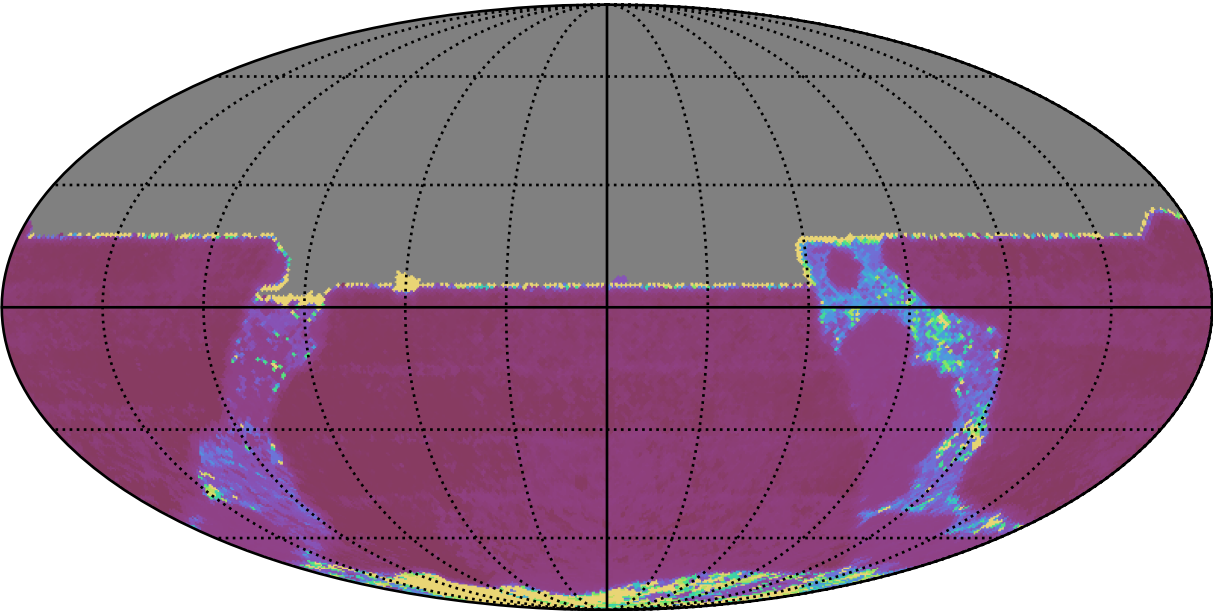
too_elab_2yr_r64_d3_ugrizy_v3.4_10yrs All sky y band: Median Inter-Night Gap
