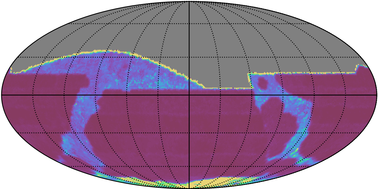
too_elab_2yr_r64_d3_ugrizy_v3.4_10yrs All sky r band: Median Inter-Night Gap
