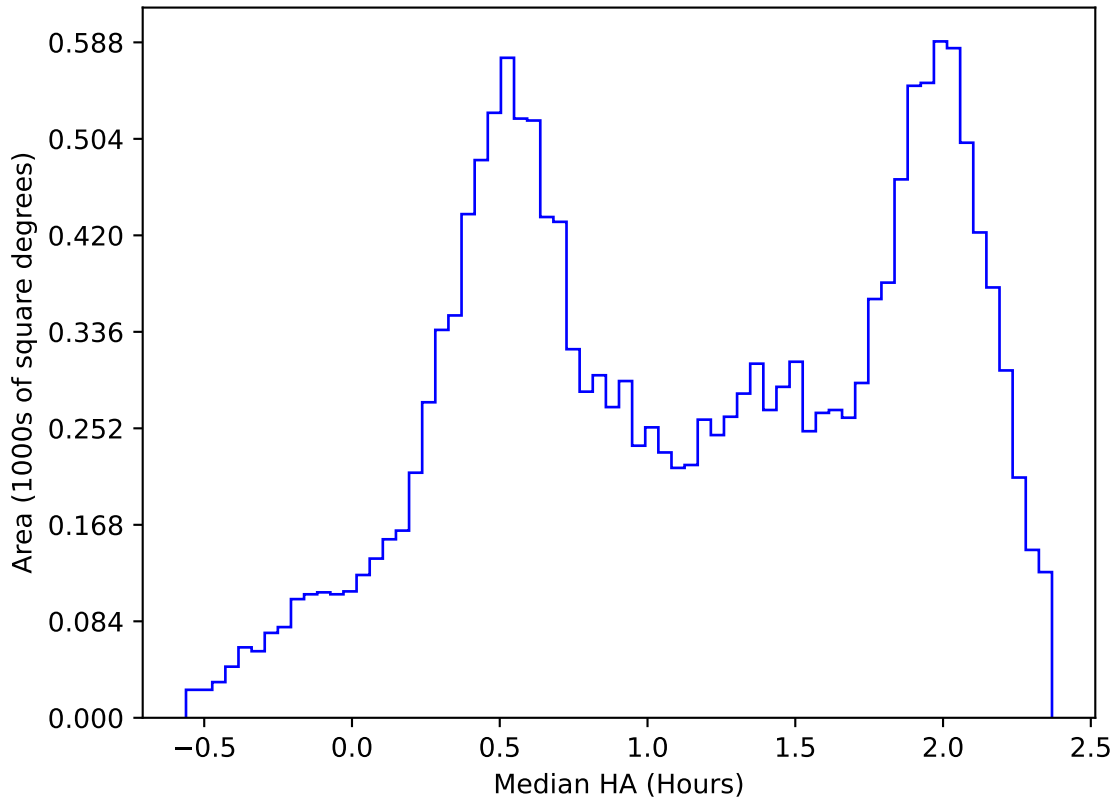
too_elab_2yr_r64_d3_ugrizy_v3.4_10yrs WFD z band: Median HA
