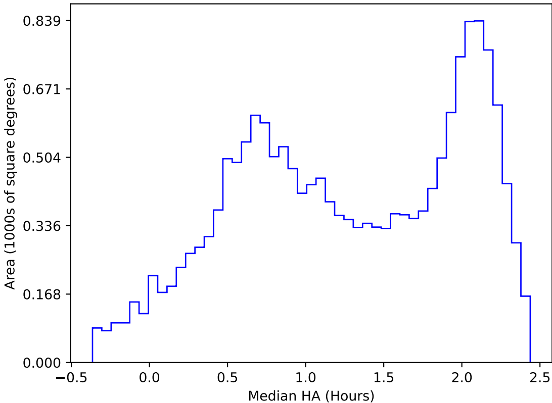
too_elab_2yr_r64_d3_ugrizy_v3.4_10yrs WFD y band: Median HA
