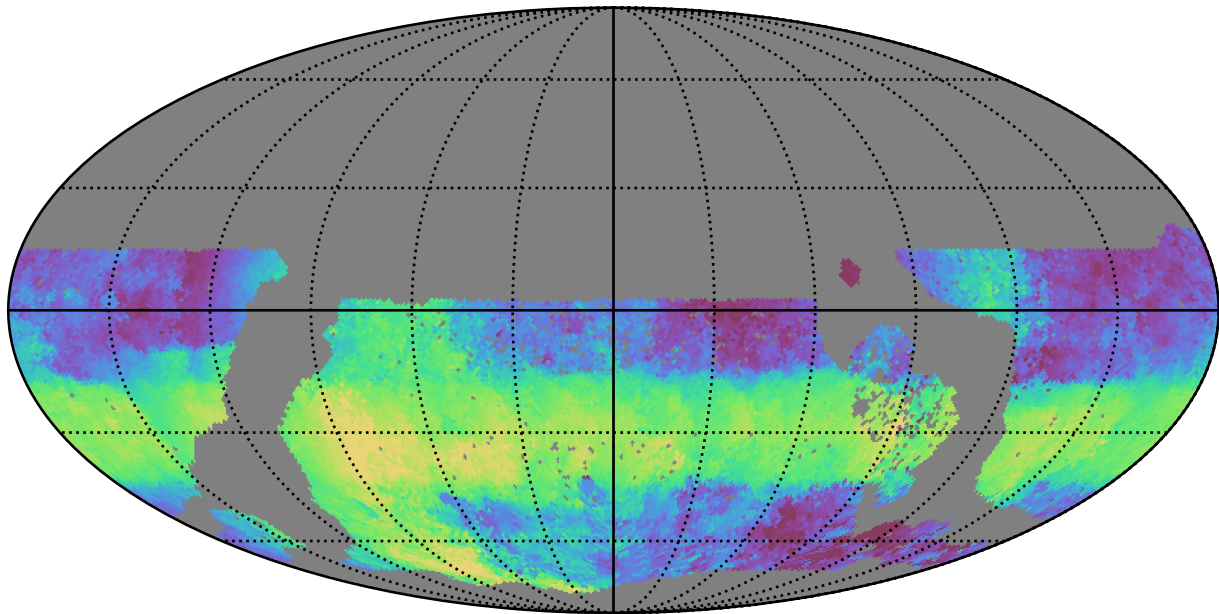
too_elab_2yr_r64_d3_ugrizy_v3.4_10yrs WFD u band: Median HA
