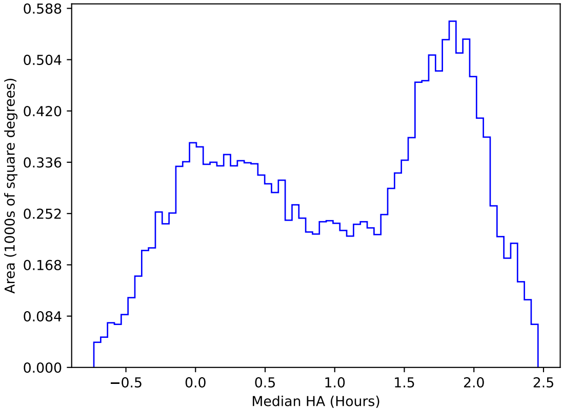
too_elab_2yr_r64_d3_ugrizy_v3.4_10yrs WFD u band: Median HA
