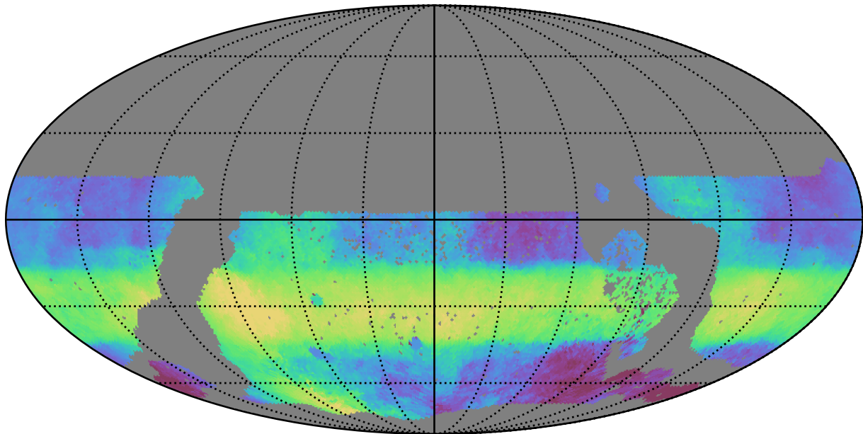
too_elab_2yr_r64_d3_ugrizy_v3.4_10yrs WFD r band: Median HA
