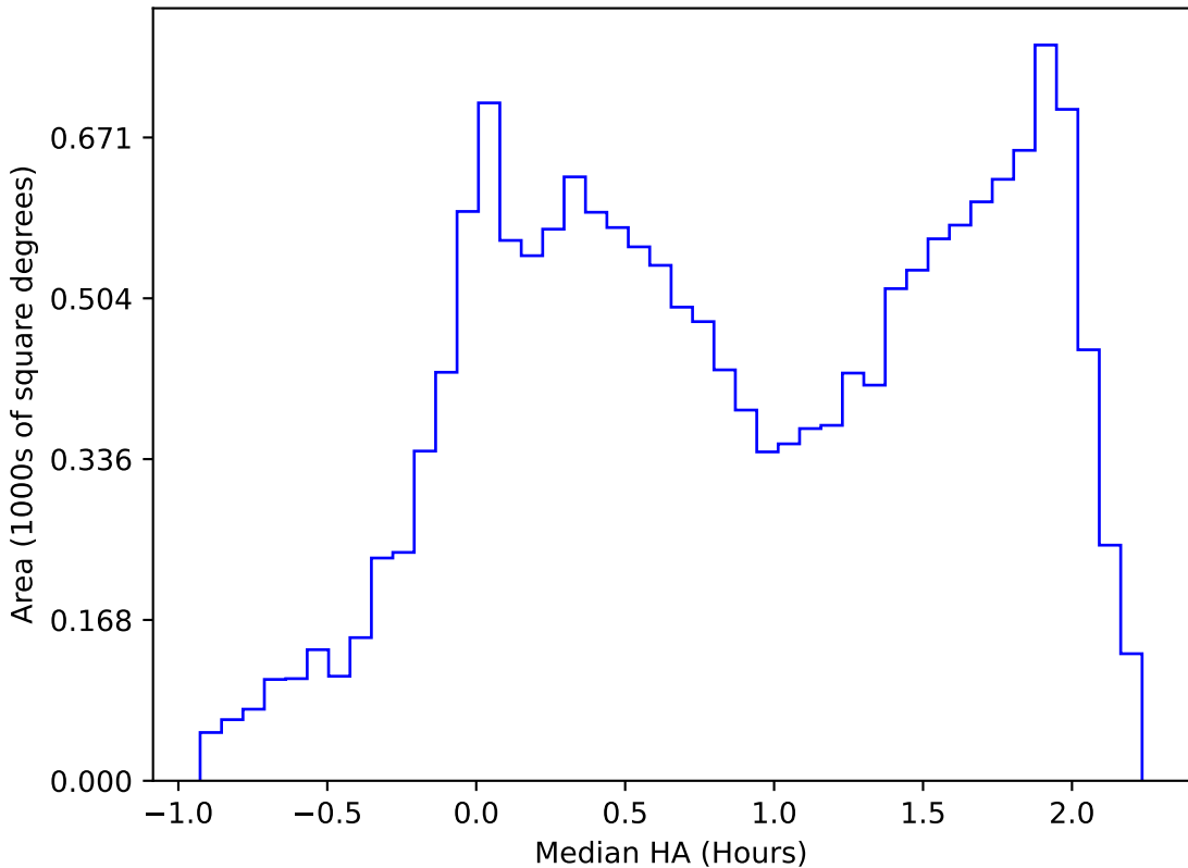
too_elab_2yr_r64_d3_ugrizy_v3.4_10yrs WFD r band: Median HA
