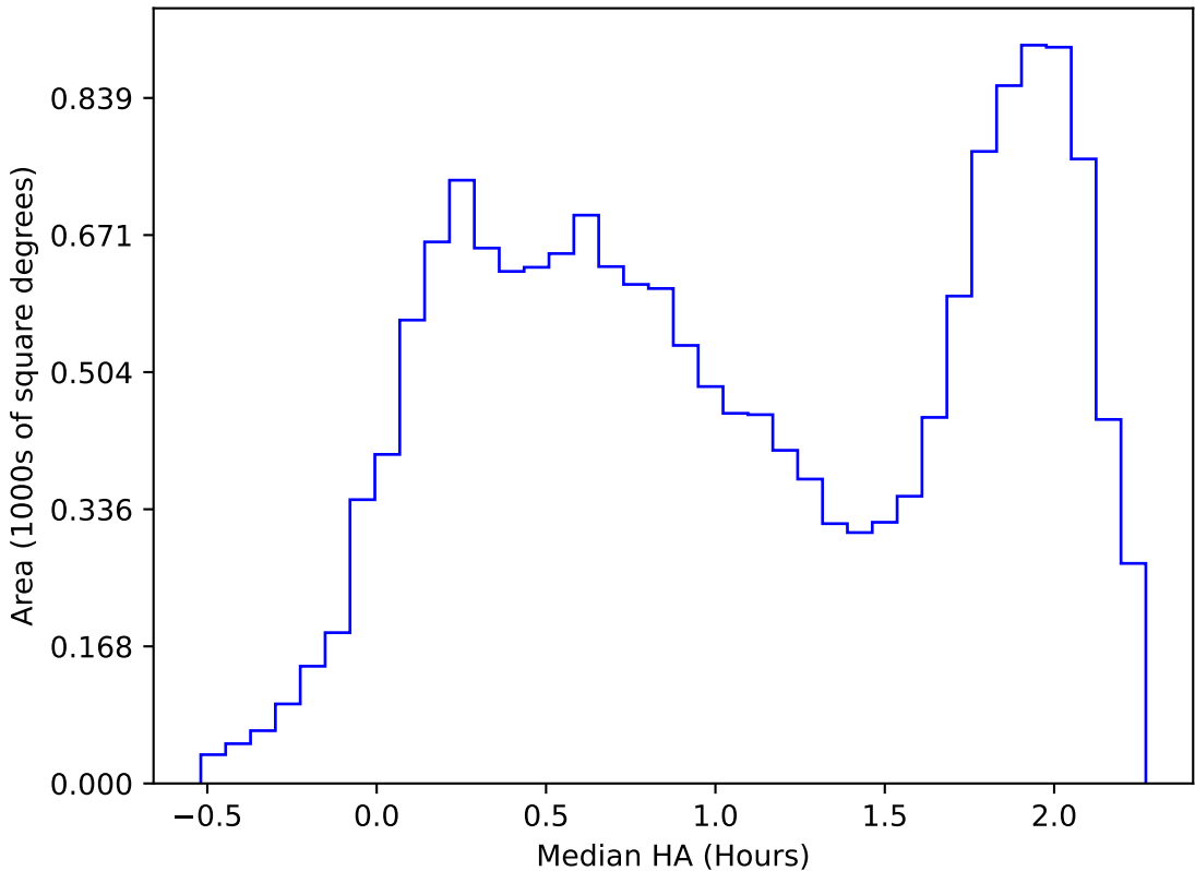
too_elab_2yr_r64_d3_ugrizy_v3.4_10yrs WFD i band: Median HA
