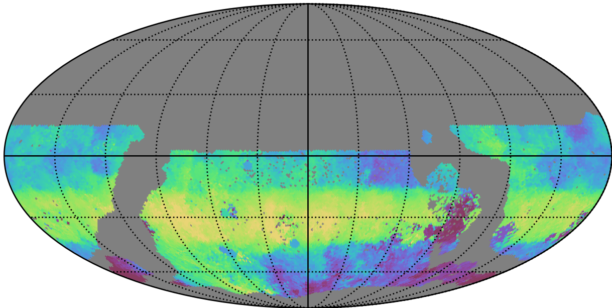
too_elab_2yr_r64_d3_ugrizy_v3.4_10yrs WFD g band: Median HA
