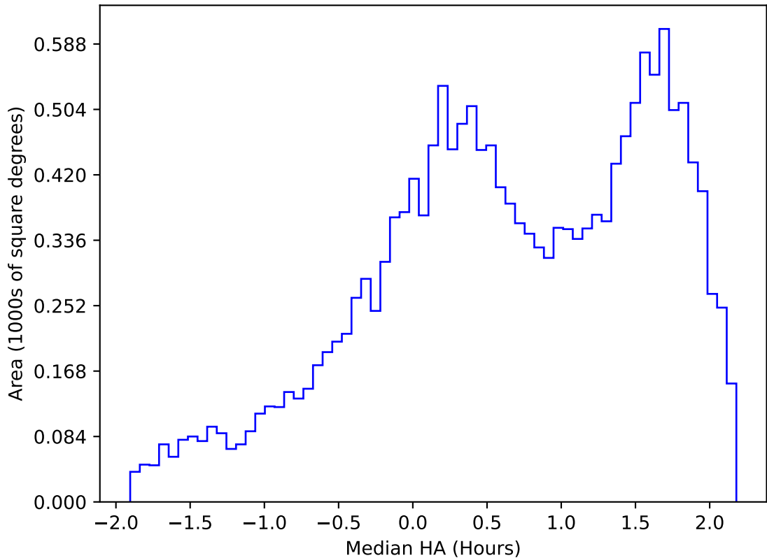
too_elab_2yr_r64_d3_ugrizy_v3.4_10yrs WFD g band: Median HA
