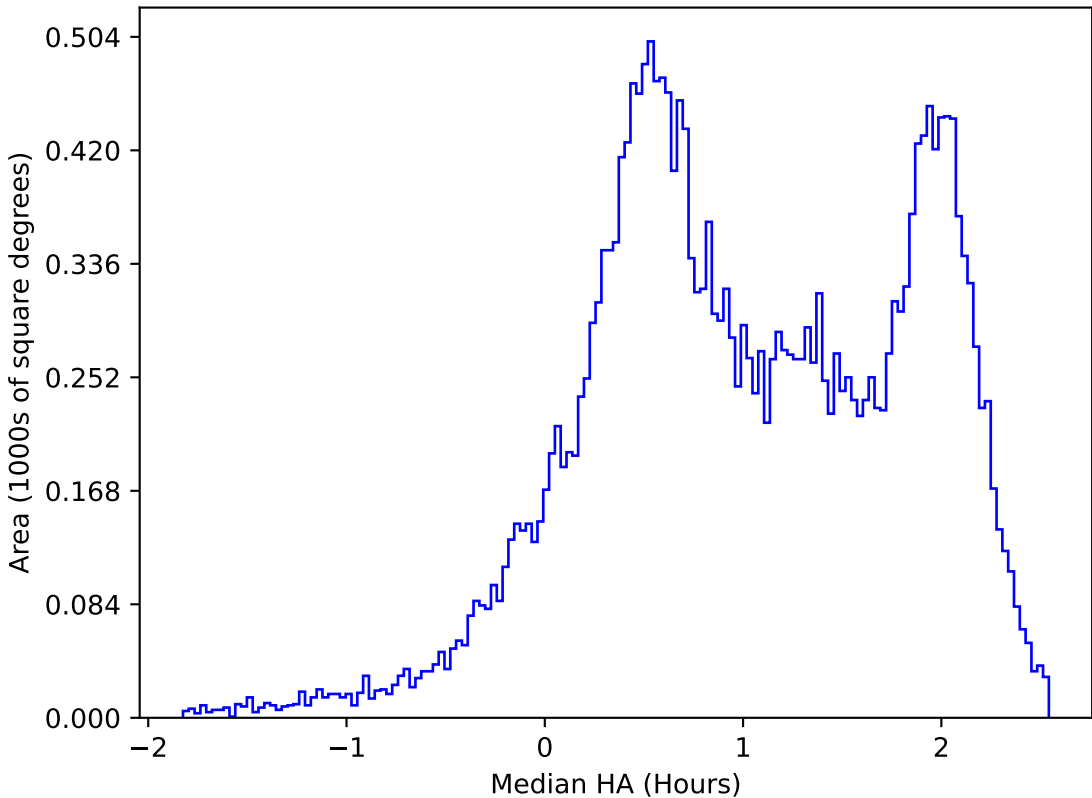
too_elab_2yr_r64_d3_ugrizy_v3.4_10yrs All sky z band: Median HA
