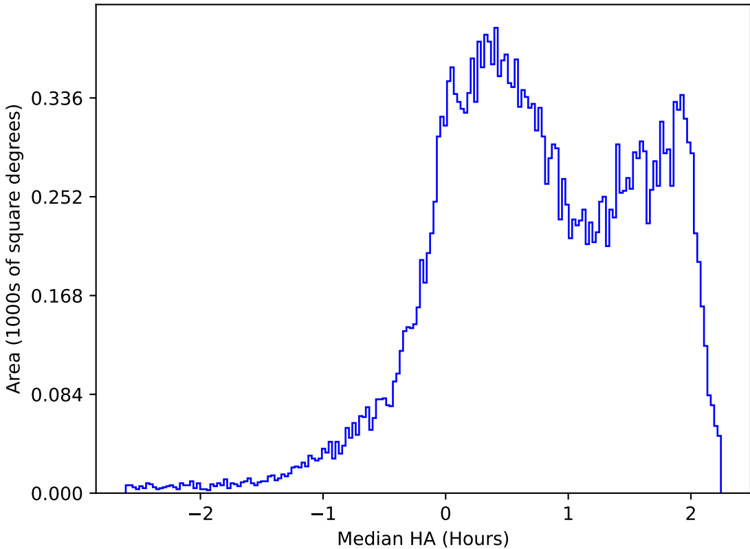
too_elab_2yr_r64_d3_ugrizy_v3.4_10yrs All sky r band: Median HA
