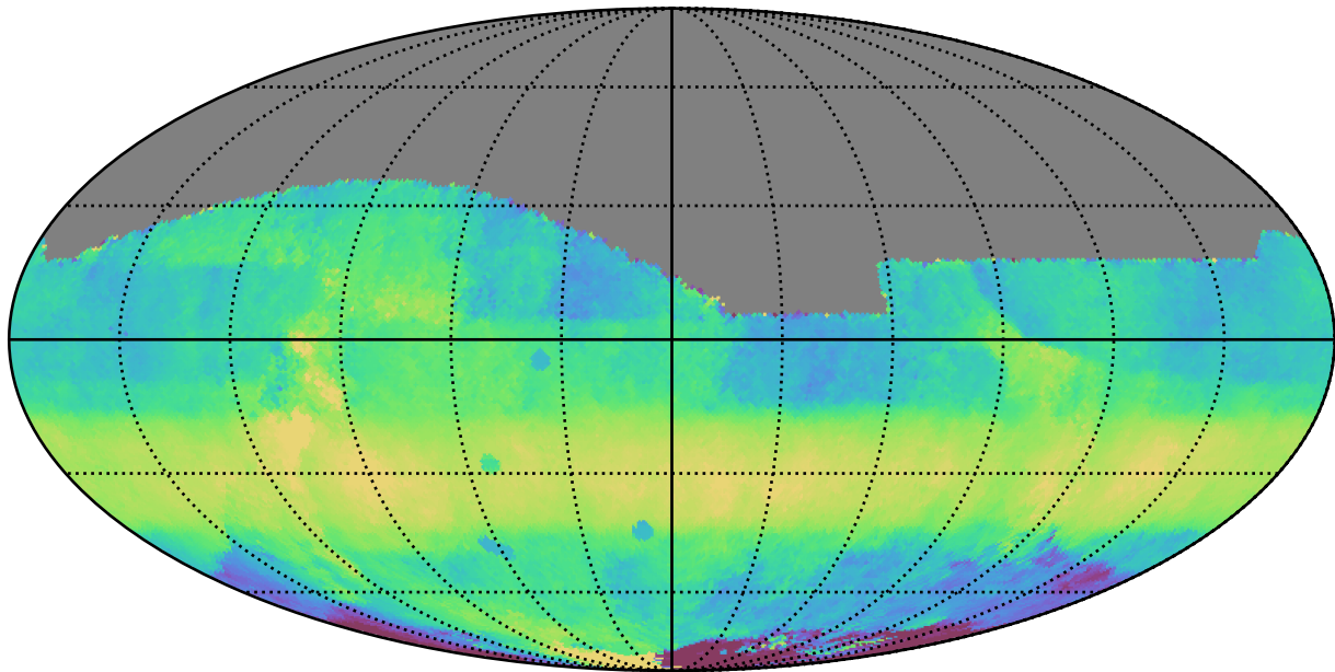
too_elab_2yr_r64_d3_ugrizy_v3.4_10yrs All sky i band: Median HA
