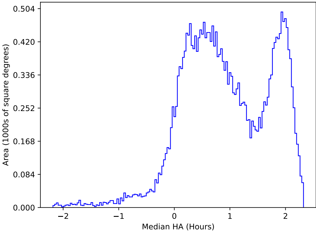
too_elab_2yr_r64_d3_ugrizy_v3.4_10yrs All sky i band: Median HA
