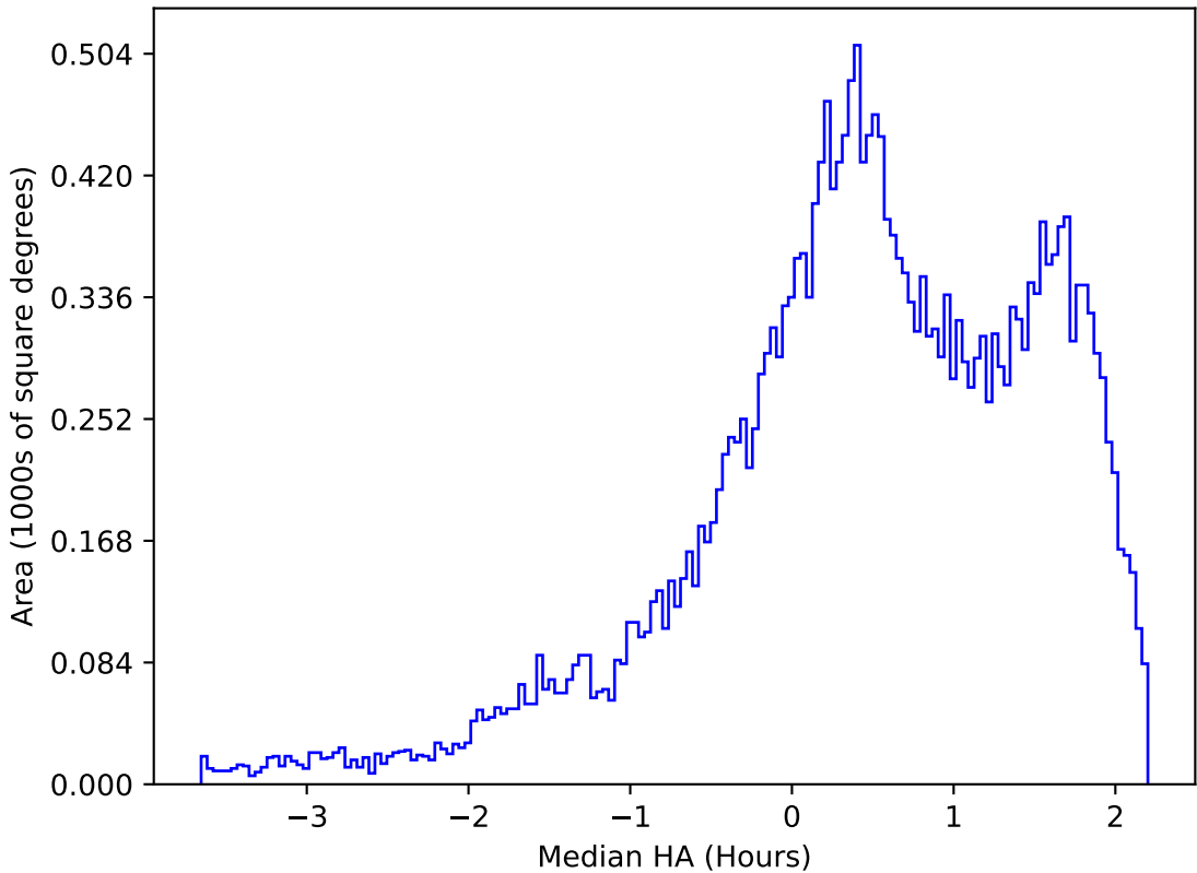
too_elab_2yr_r64_d3_ugrizy_v3.4_10yrs All sky g band: Median HA
