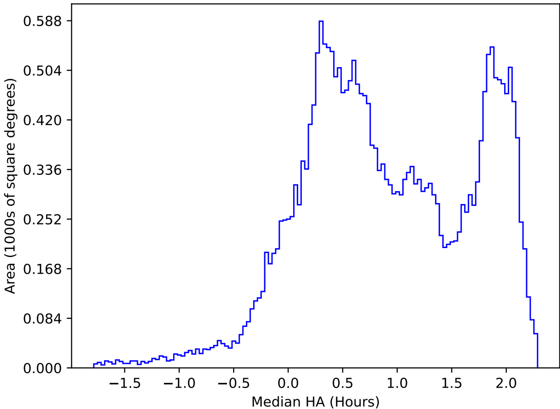
too_elab_2yr_r64_d3_ugrizy_v3.4_10yrs All sky all bands: Median HA
