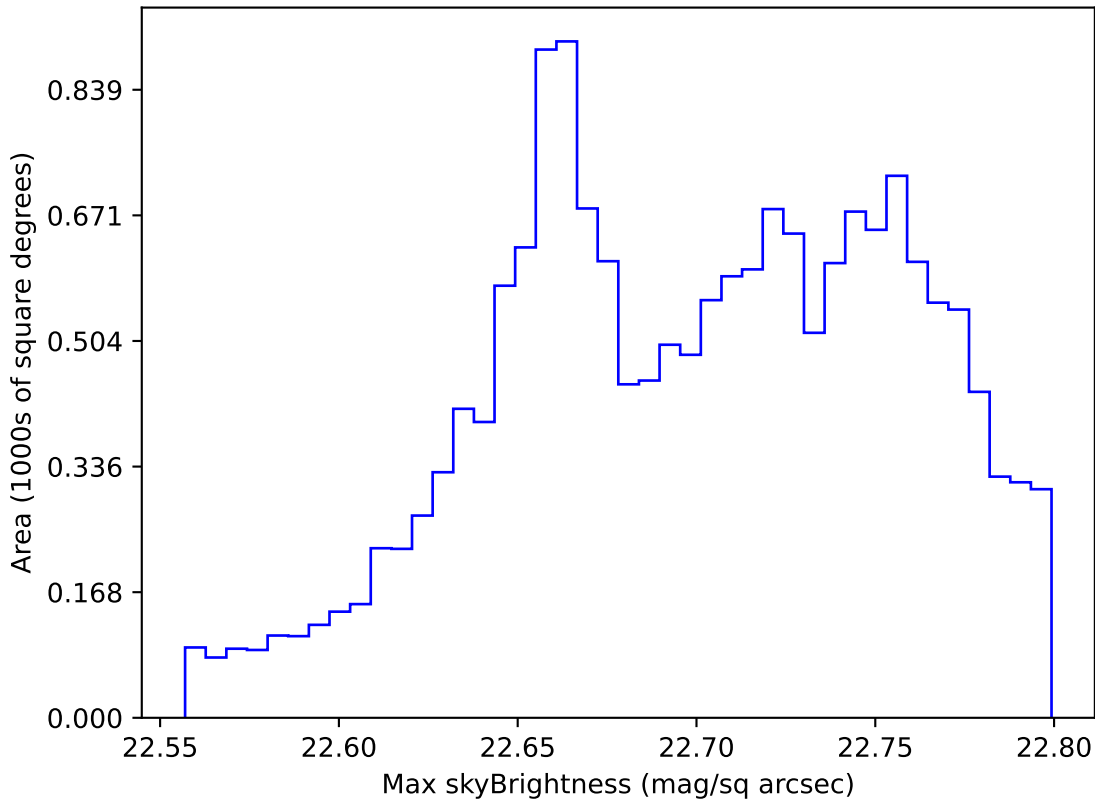
too_elab_2yr_r64_d3_ugrizy_v3.4_10yrs WFD all bands: Max skyBrightness
