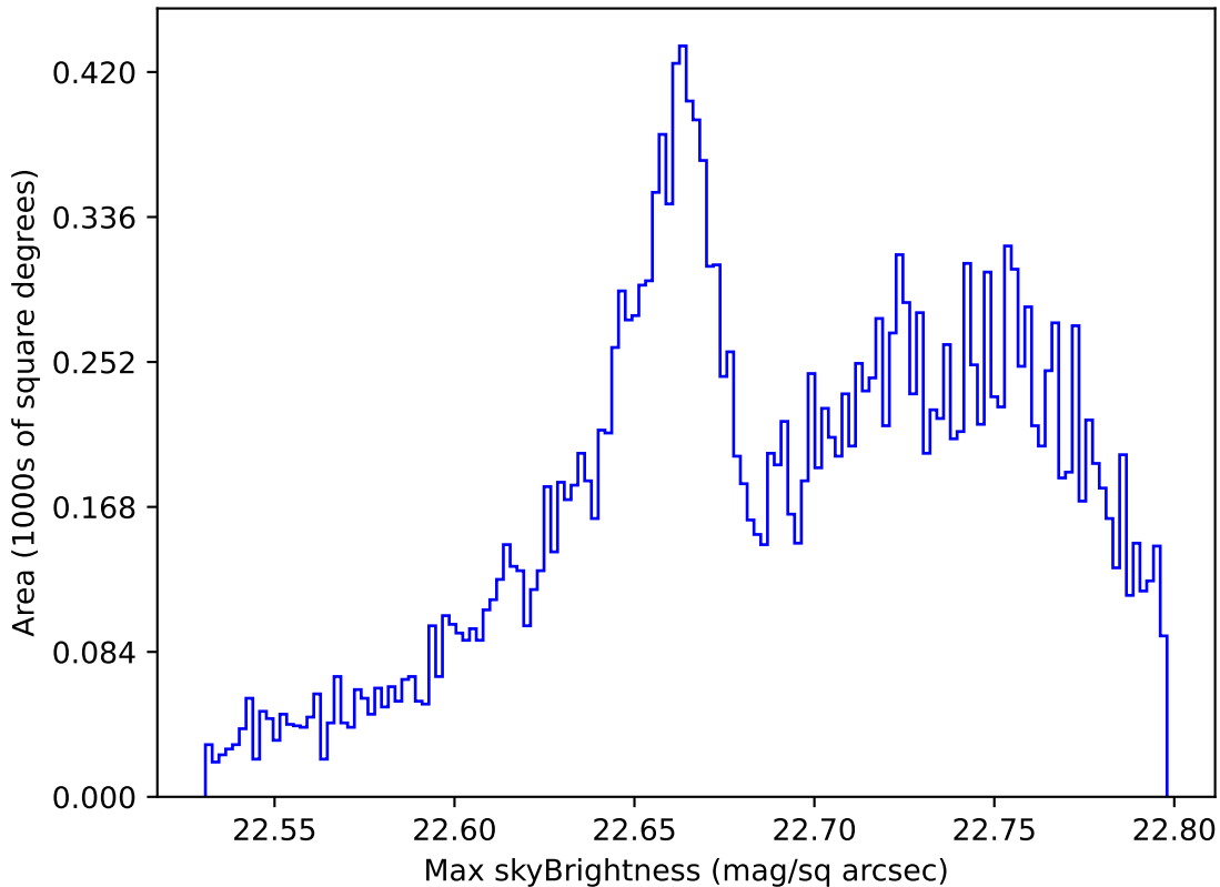
too_elab_2yr_r64_d3_ugrizy_v3.4_10yrs All sky u band: Max skyBrightness
