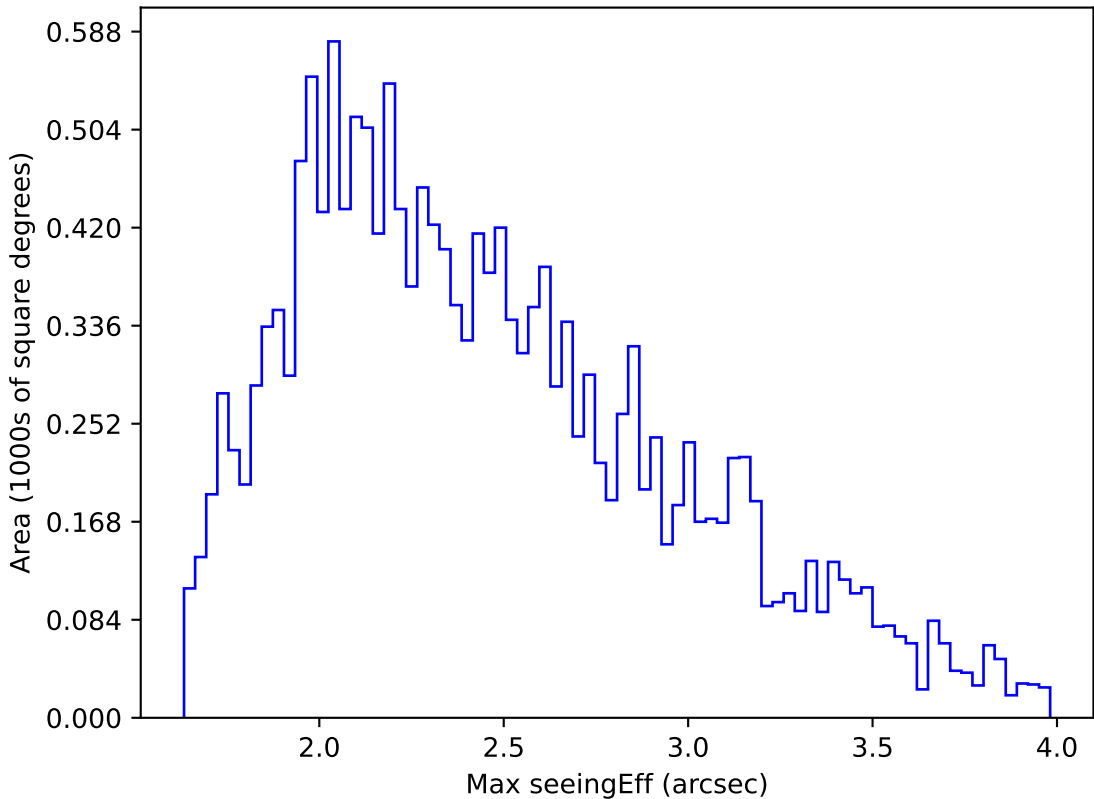
too_elab_2yr_r64_d3_ugrizy_v3.4_10yrs WFD g band: Max seeingEff
