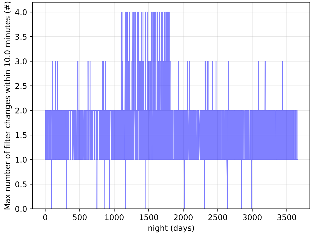
too_elab_2yr_r64_d3_ugrizy_v3.4_10yrs Per Night: Max number of filter changes within 10.0 minutes
