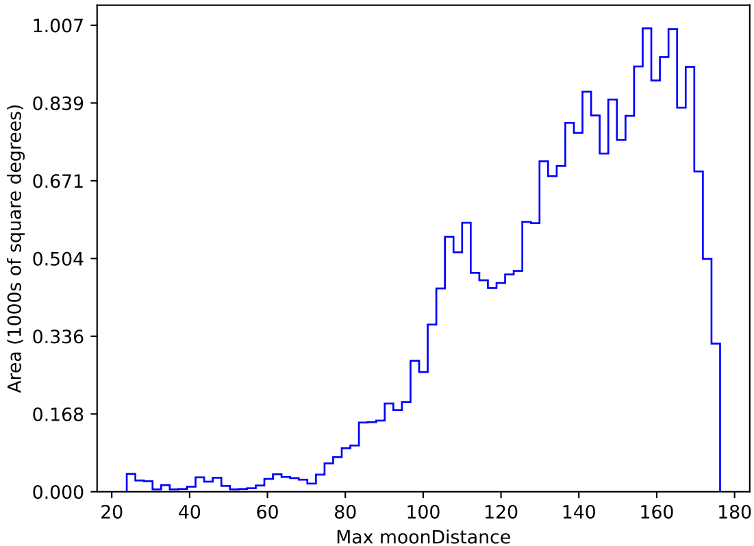
too_elab_2yr_r64_d3_ugrizy_v3.4_10yrs All sky y band: Max moonDistance
