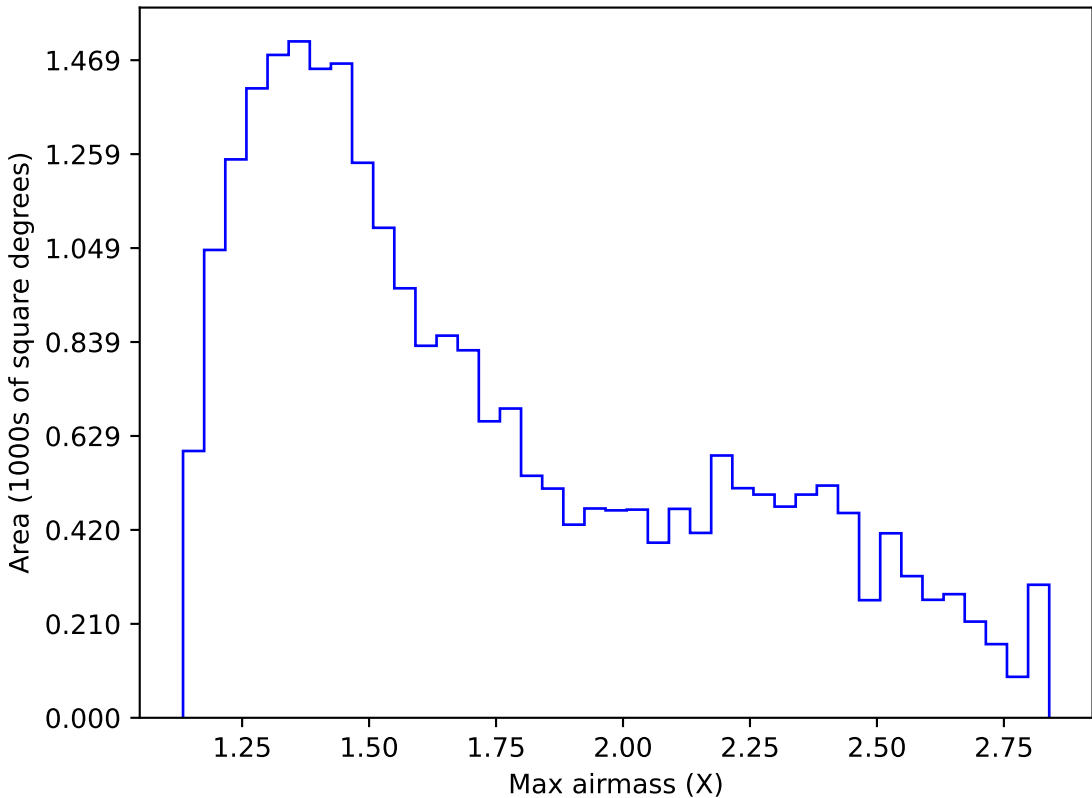
too_elab_2yr_r64_d3_ugrizy_v3.4_10yrs Yr 1 z band: Max airmass
