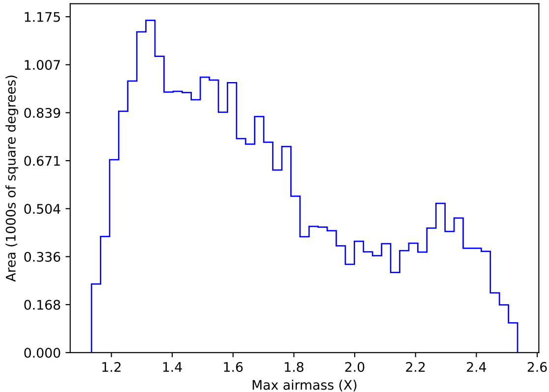
too_elab_2yr_r64_d3_ugrizy_v3.4_10yrs Yr 1 r band: Max airmass
