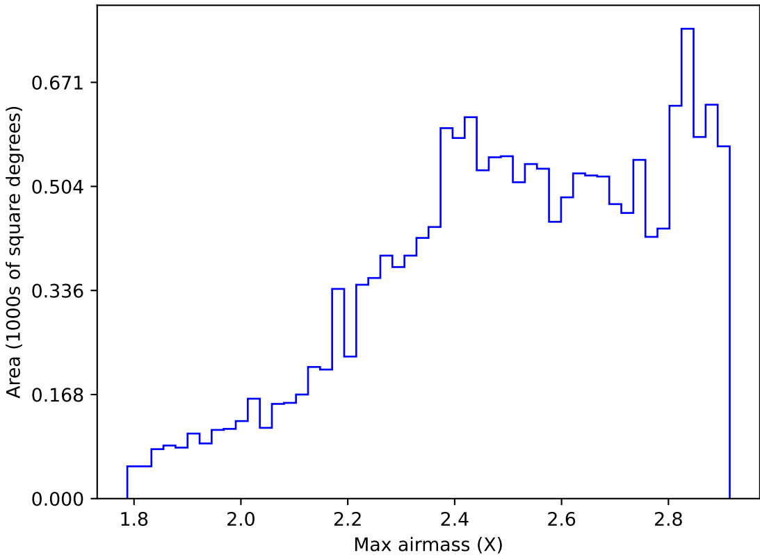
too_elab_2yr_r64_d3_ugrizy_v3.4_10yrs WFD z band: Max airmass
