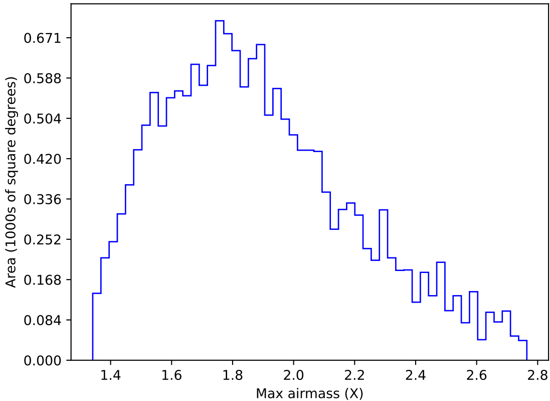
too_elab_2yr_r64_d3_ugrizy_v3.4_10yrs WFD u band: Max airmass
