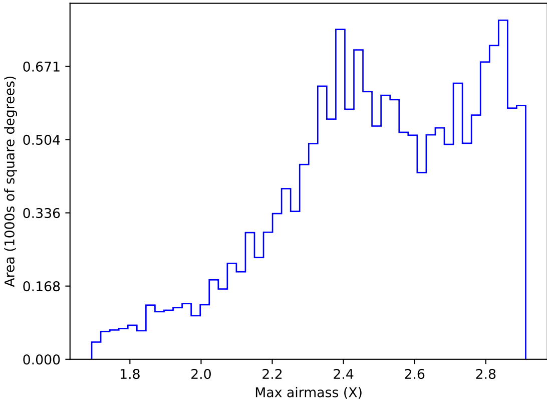
too_elab_2yr_r64_d3_ugrizy_v3.4_10yrs WFD i band: Max airmass
