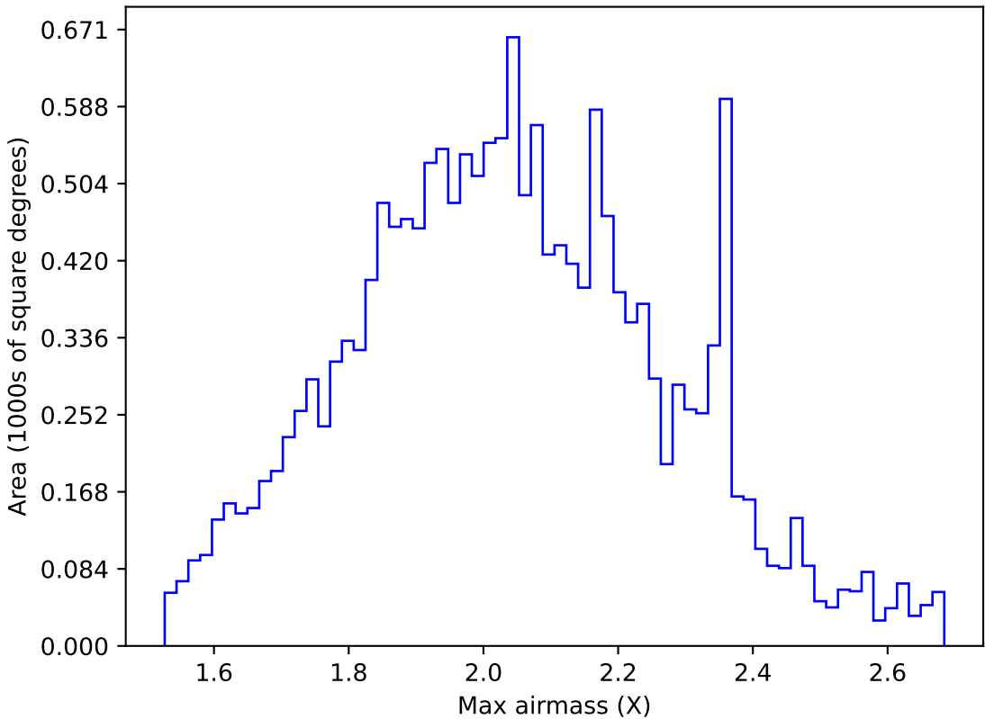
too_elab_2yr_r64_d3_ugrizy_v3.4_10yrs WFD g band: Max airmass
