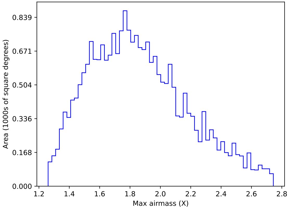
too_elab_2yr_r64_d3_ugrizy_v3.4_10yrs All sky u band: Max airmass
