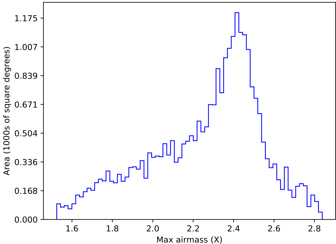
too_elab_2yr_r64_d3_ugrizy_v3.4_10yrs All sky r band: Max airmass
