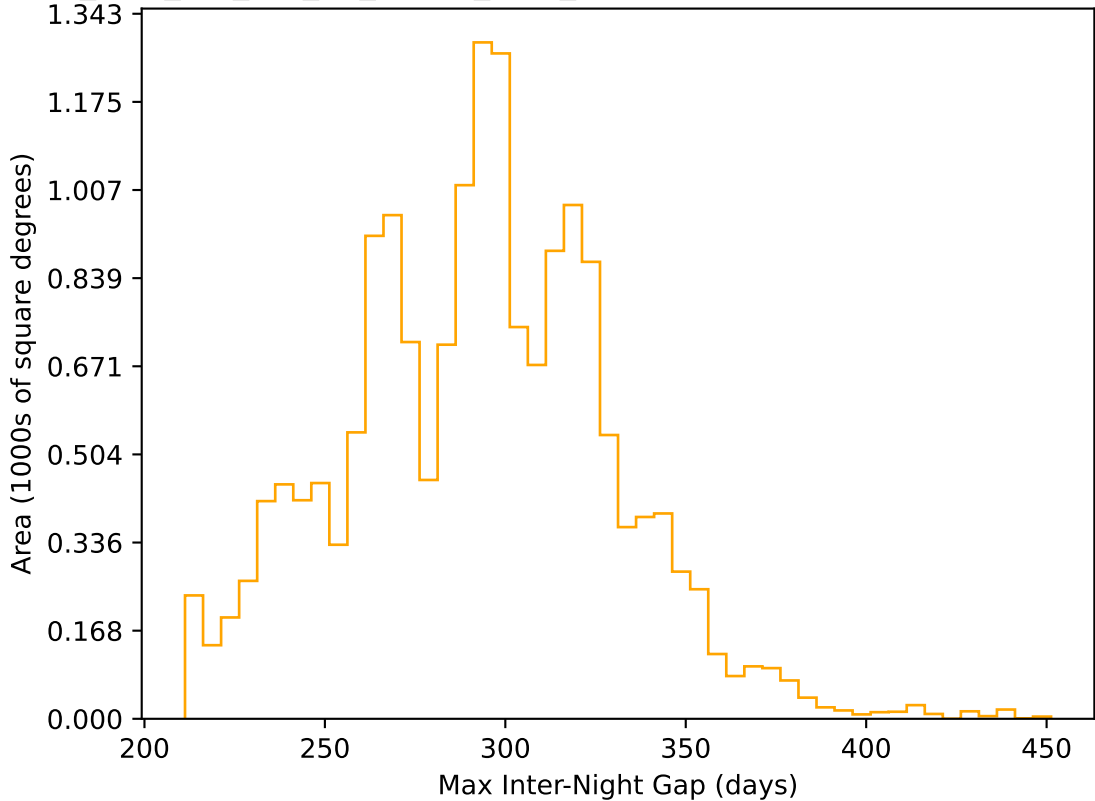
too_elab_2yr_r64_d3_ugrizy_v3.4_10yrs WFD r band: Max Inter-Night Gap
