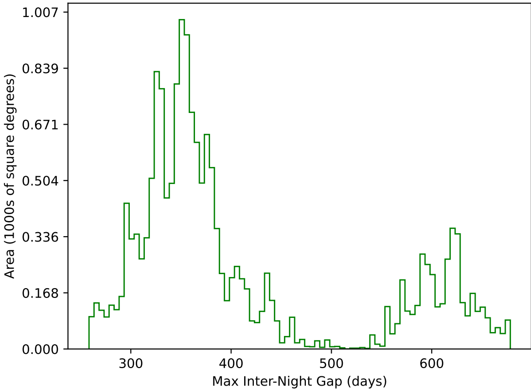
too_elab_2yr_r64_d3_ugrizy_v3.4_10yrs WFD g band: Max Inter-Night Gap
