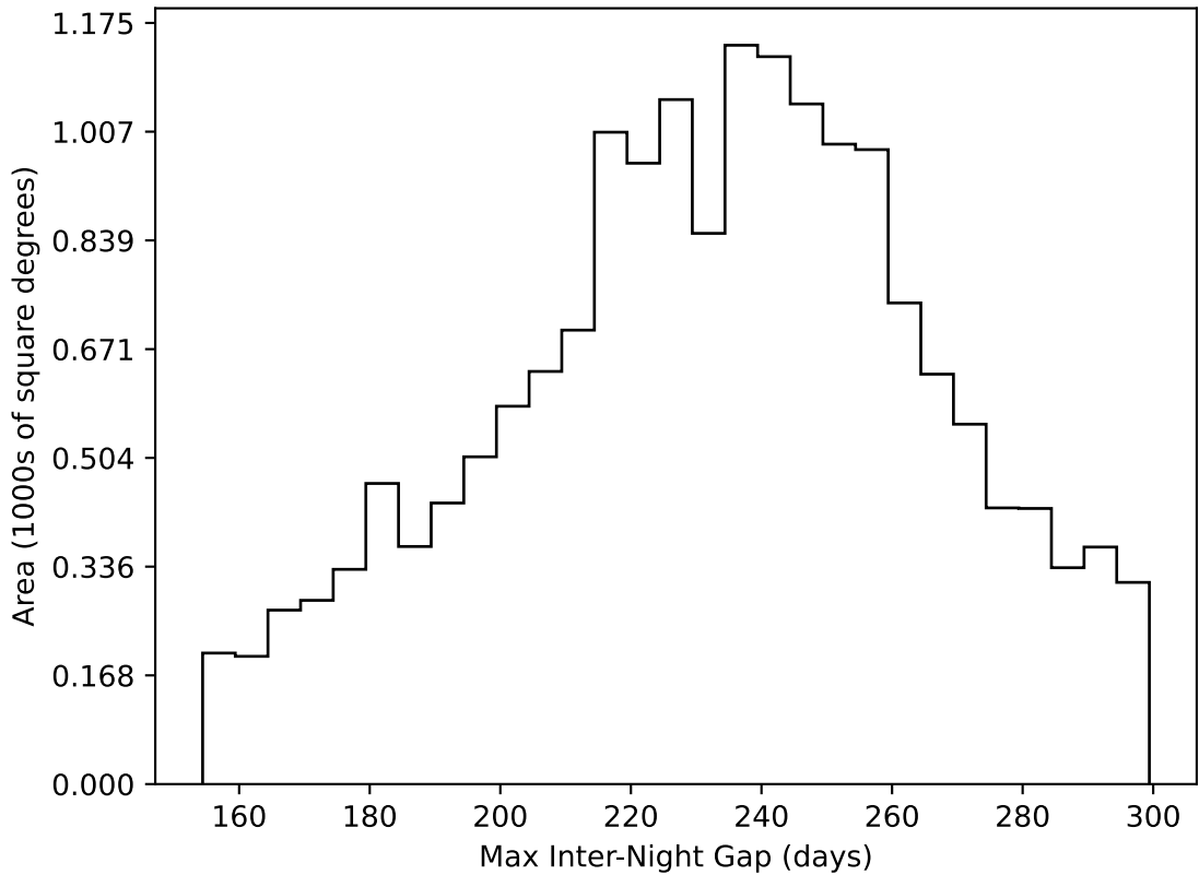
too_elab_2yr_r64_d3_ugrizy_v3.4_10yrs WFD all bands: Max Inter-Night Gap
