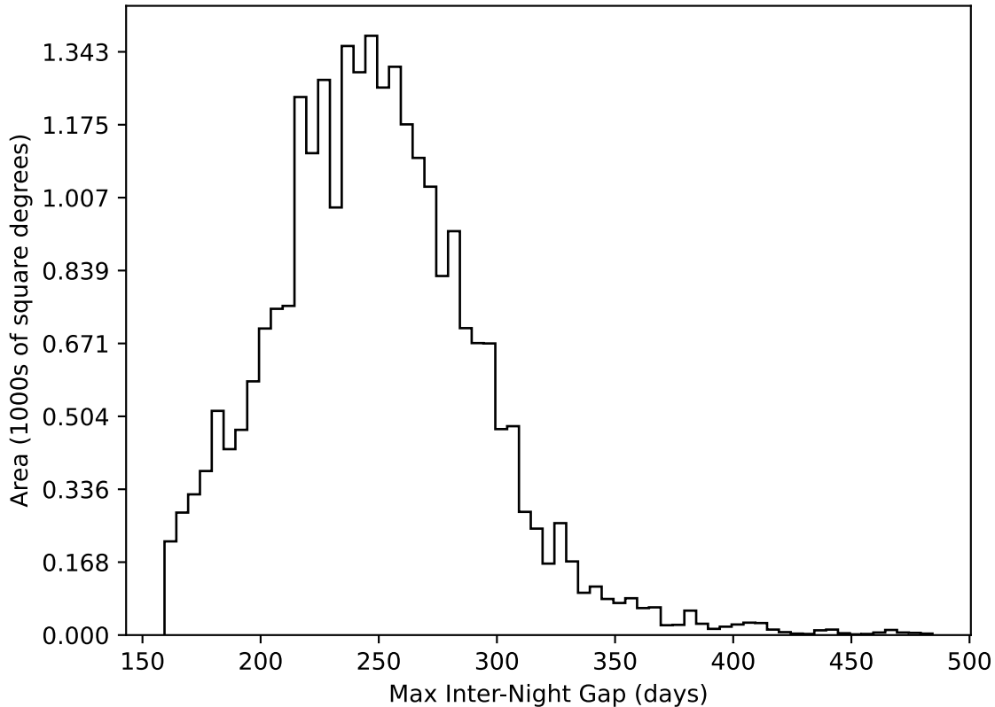
too_elab_2yr_r64_d3_ugrizy_v3.4_10yrs All sky all bands: Max Inter-Night Gap
