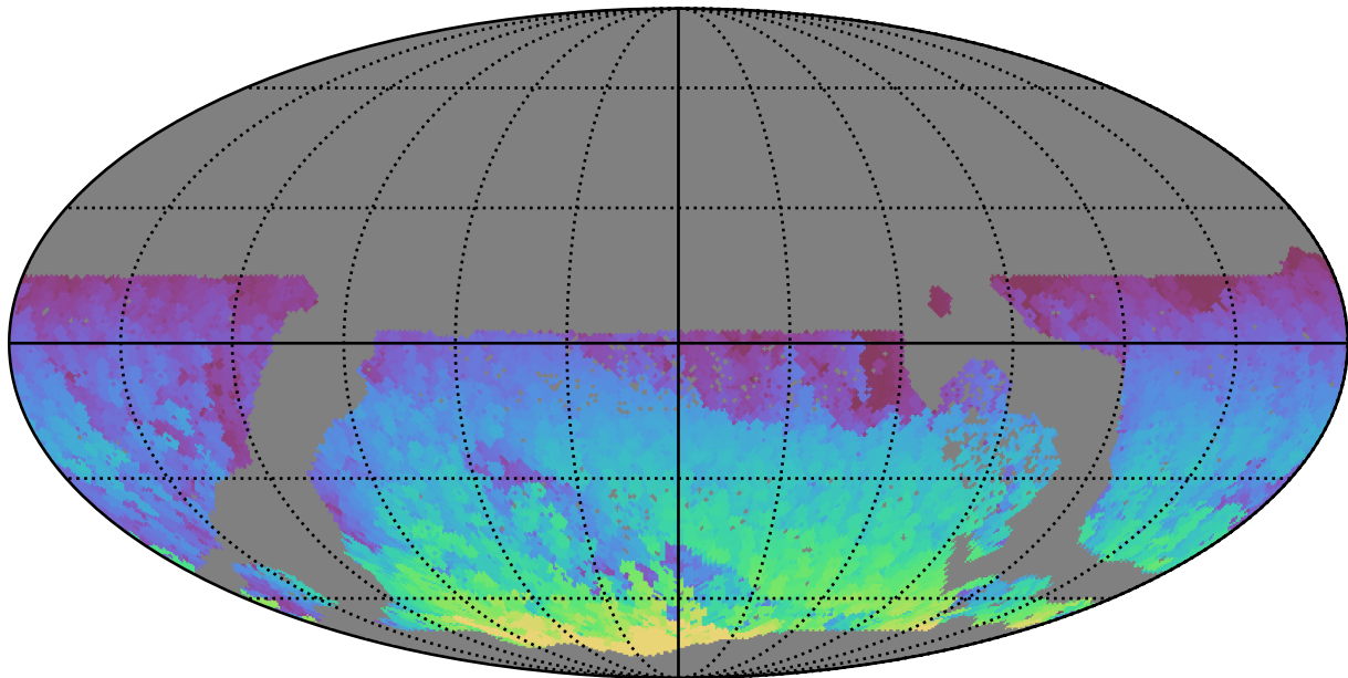
too_elab_2yr_r64_d3_ugrizy_v3.4_10yrs WFD z band: Max HA
