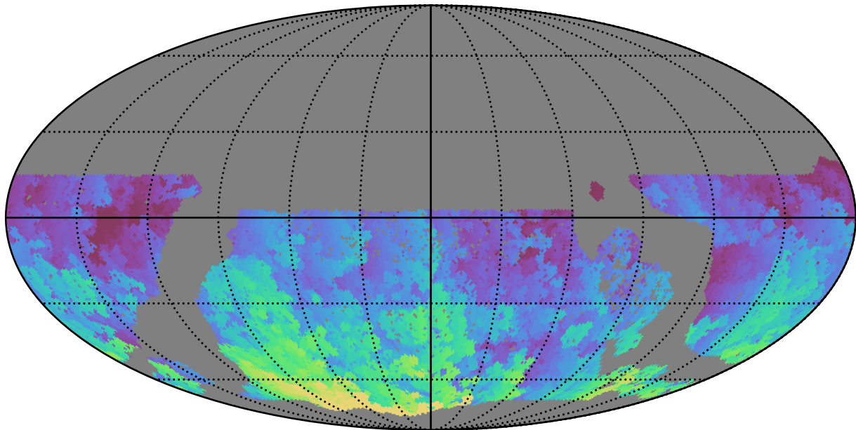
too_elab_2yr_r64_d3_ugrizy_v3.4_10yrs WFD u band: Max HA
