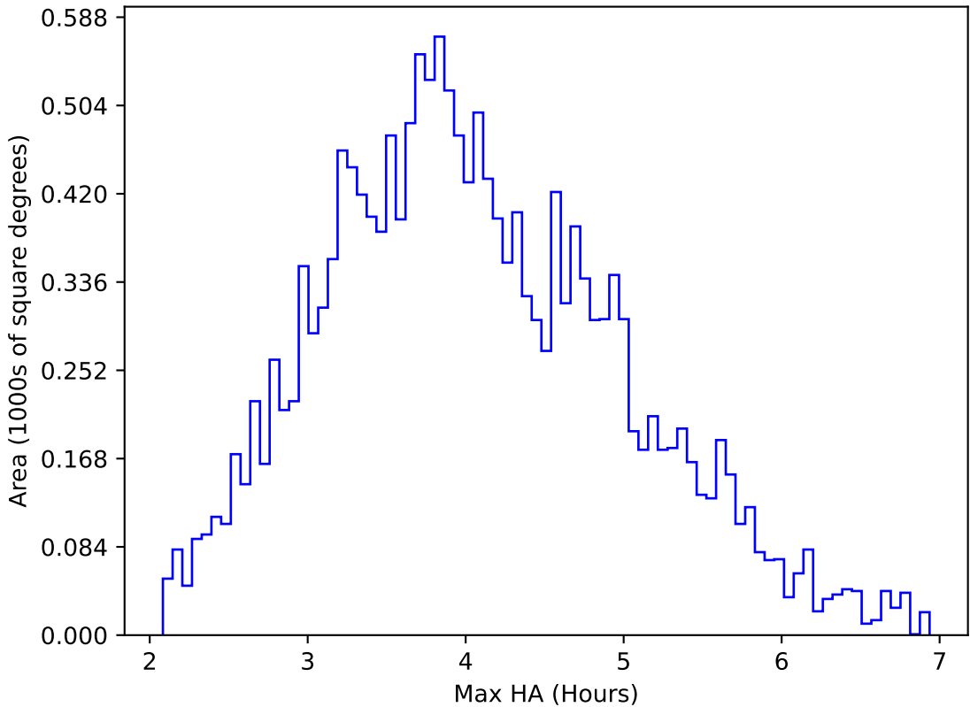
too_elab_2yr_r64_d3_ugrizy_v3.4_10yrs WFD u band: Max HA
