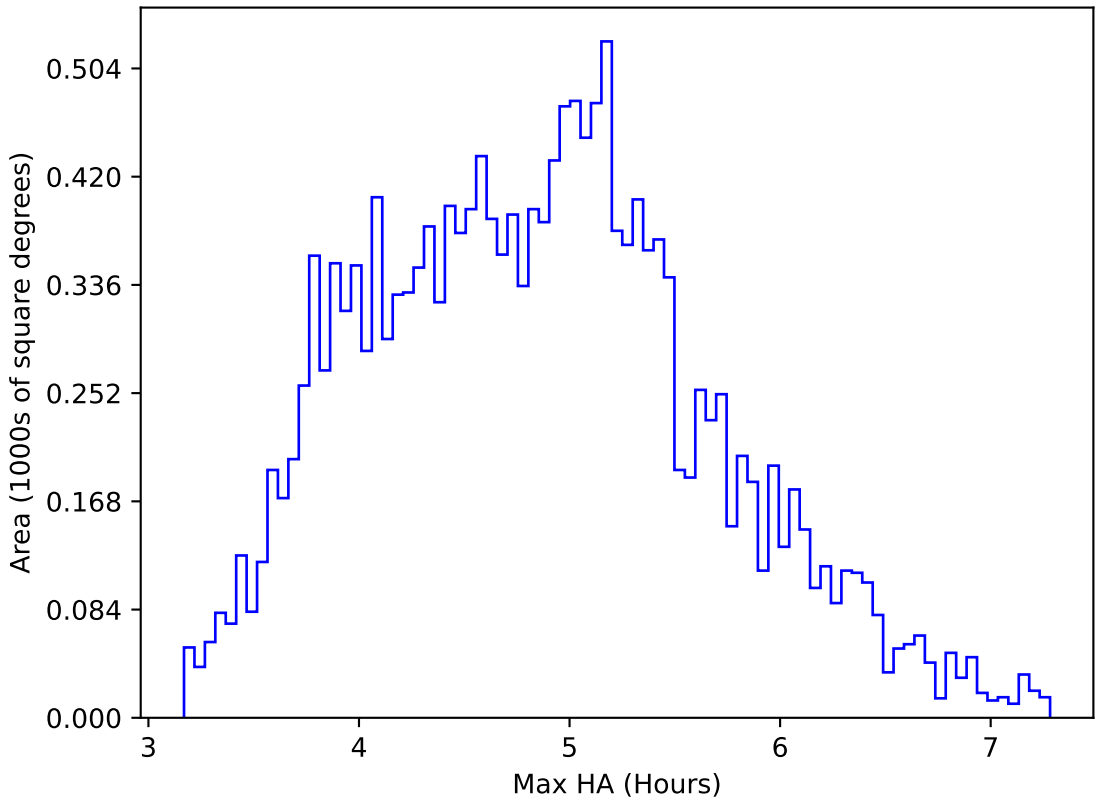
too_elab_2yr_r64_d3_ugrizy_v3.4_10yrs WFD i band: Max HA
