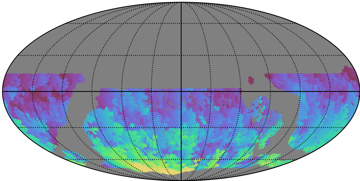
too_elab_2yr_r64_d3_ugrizy_v3.4_10yrs WFD g band: Max HA
