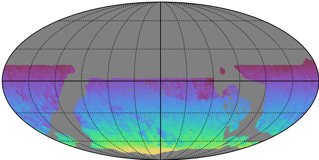
too_elab_2yr_r64_d3_ugrizy_v3.4_10yrs WFD all bands: Max HA
