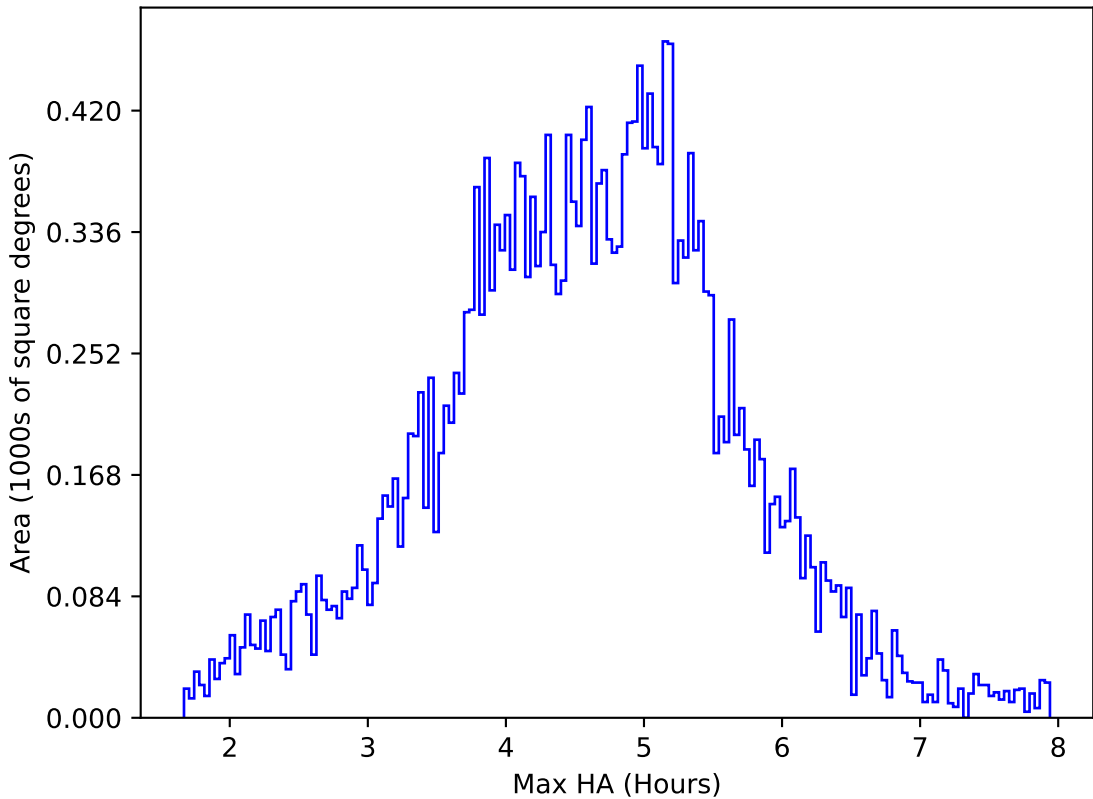
too_elab_2yr_r64_d3_ugrizy_v3.4_10yrs All sky i band: Max HA
