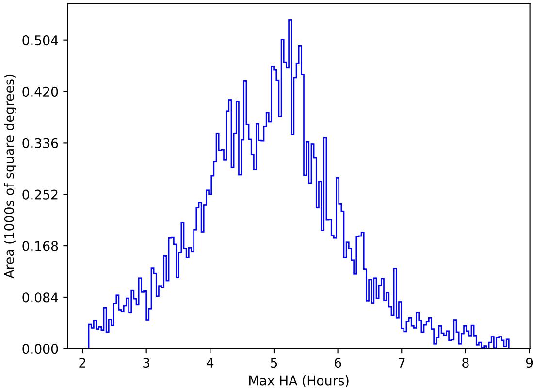
too_elab_2yr_r64_d3_ugrizy_v3.4_10yrs All sky all bands: Max HA
