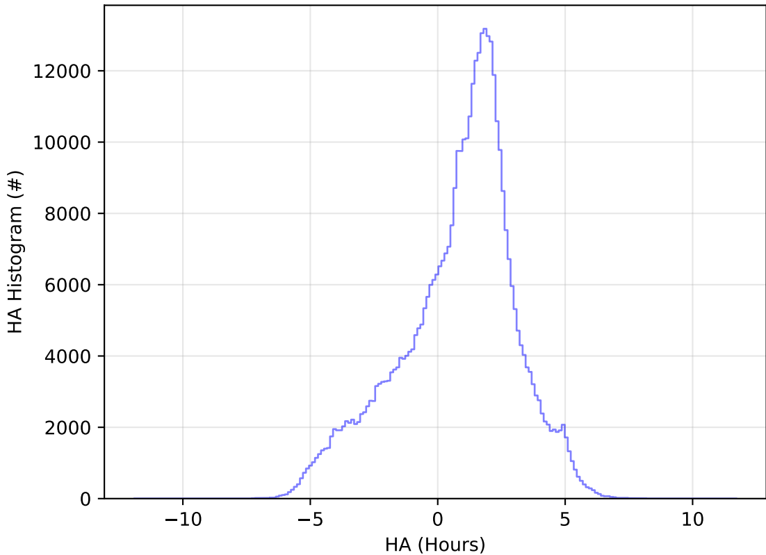
too_elab_2yr_r64_d3_ugrizy_v3.4_10yrs WFD z band: HA Histogram
