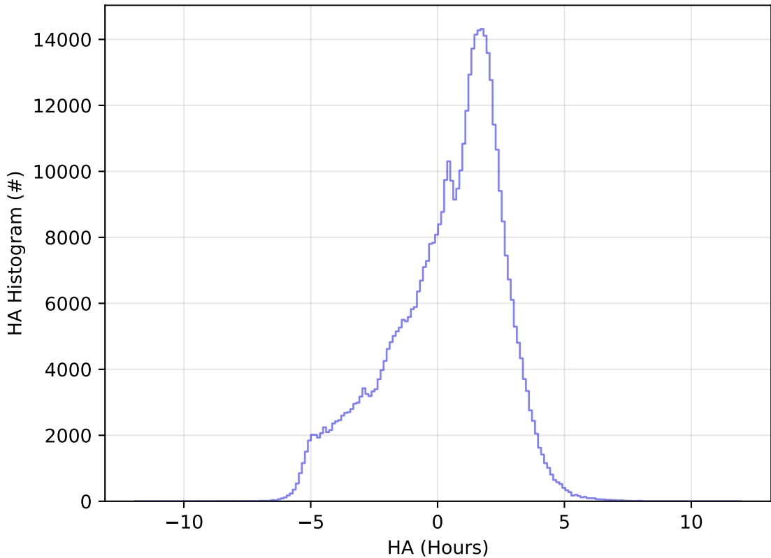
too_elab_2yr_r64_d3_ugrizy_v3.4_10yrs WFD r band: HA Histogram
