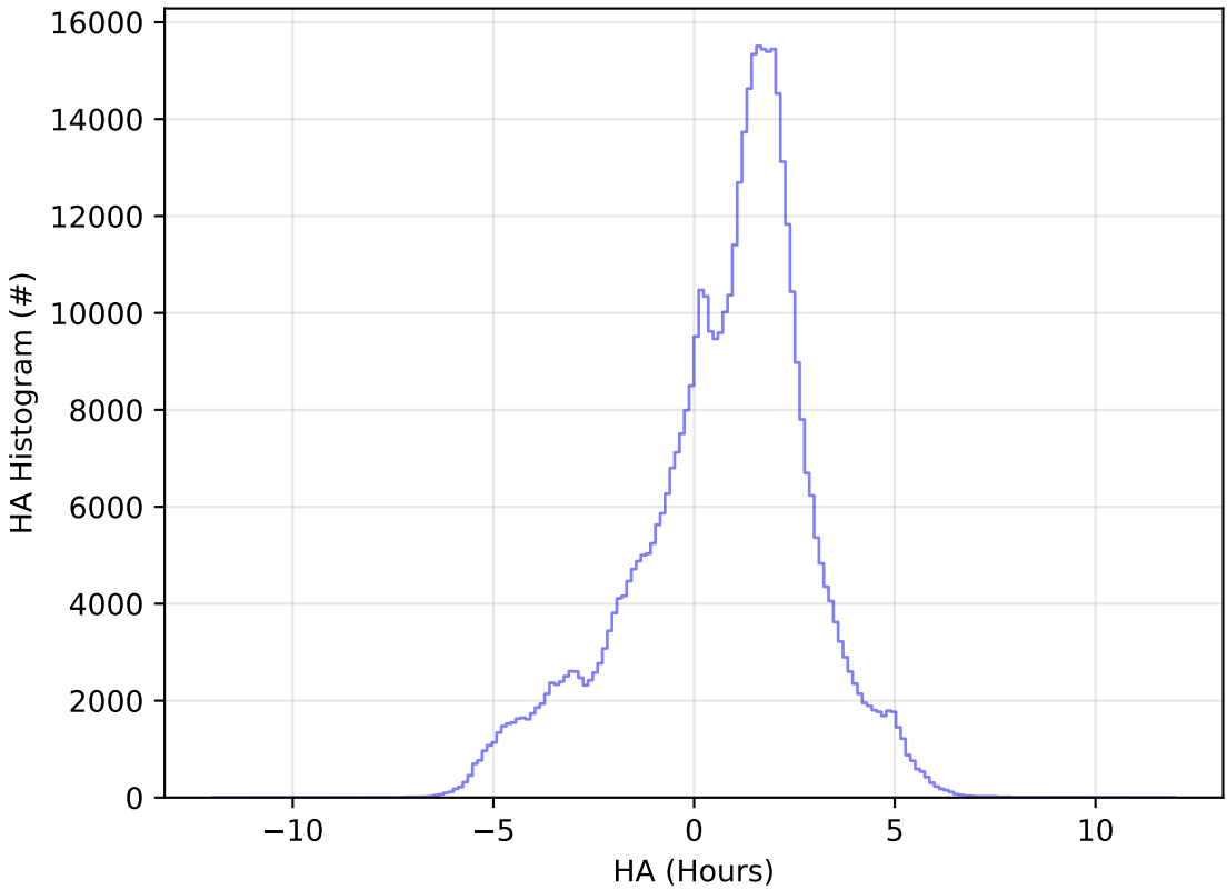
too_elab_2yr_r64_d3_ugrizy_v3.4_10yrs WFD i band: HA Histogram
