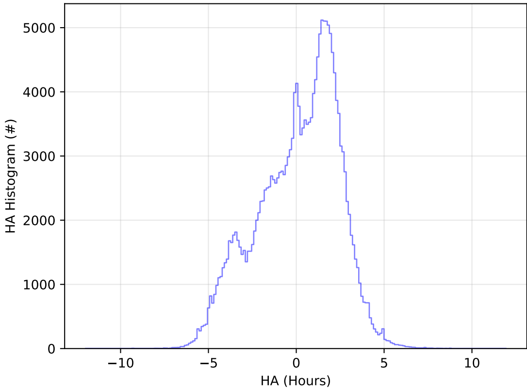
too_elab_2yr_r64_d3_ugrizy_v3.4_10yrs WFD g band: HA Histogram
